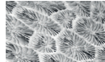
ABOVE 111 A scanning electron microscope image of bacterially cemented aggregate. With increasing magnification, the rhombohedral geometry of the calcite is revealed. Bacterial 'fossils' appear within the cement as rod-shaped voids.
